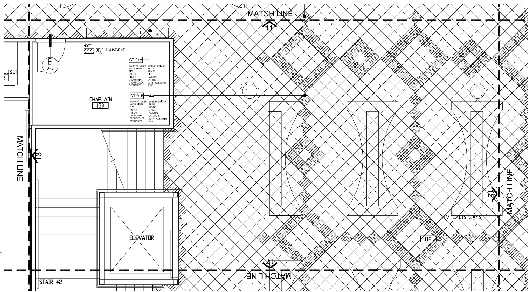
1 FIRST - PARITAL PLAN (AREA "E") 112 - DIVISON SIX DISPLAY SCALE 1/4" = 1' - 0"
